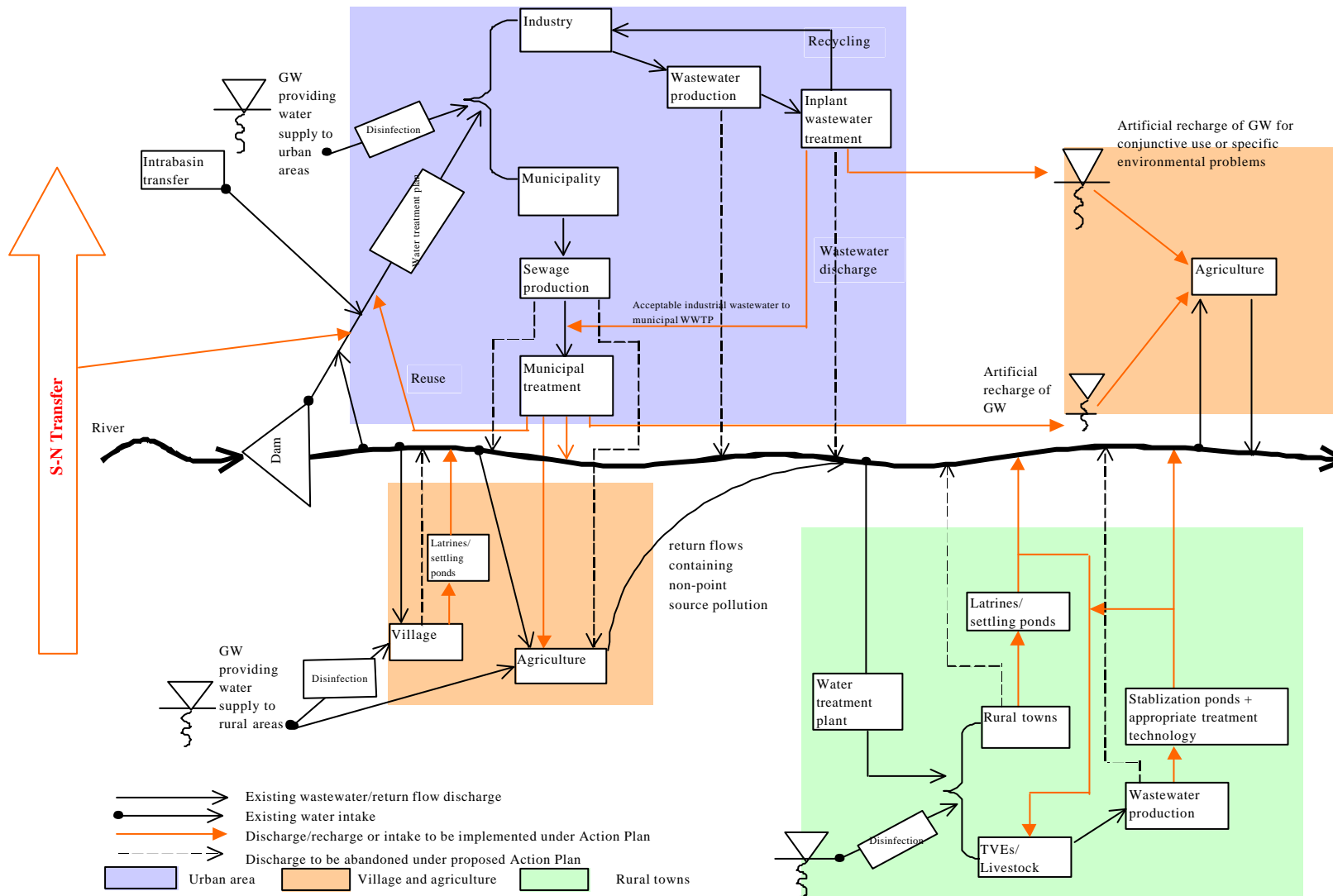
FIGURE 4.2 EXISTING AND PROPOSED INTEGRATED WATER AND WASTEWATER UTILIZATION FOR URBAN AREAS, AGRICULTURE AND RURAL TOWNS
