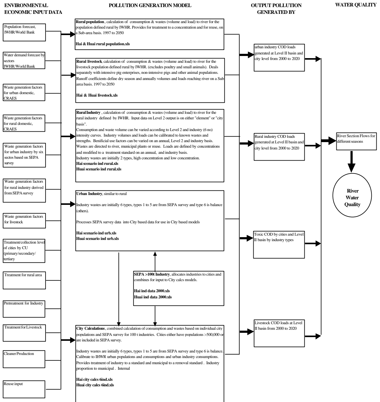
FIGURE 7.1: WATER POLLUTION MANAGEMENT MODEL DECISION SUPPORT SYSTEM (WPM-DSS)
