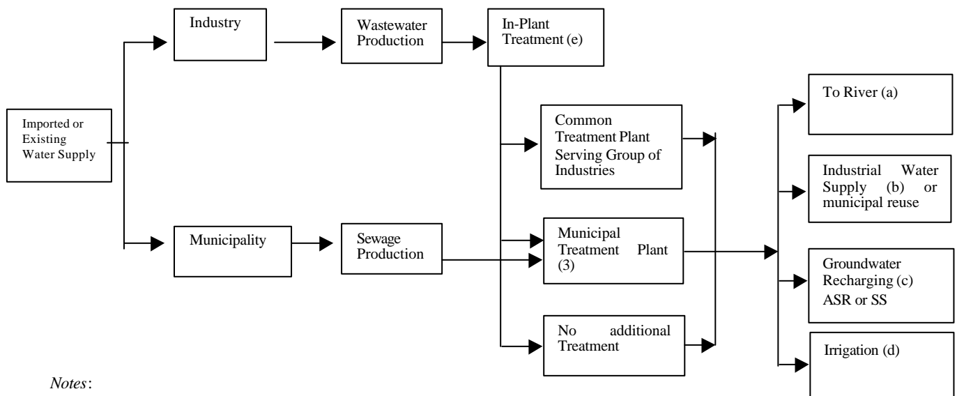
FIGURE 8.1: SCHEMATIC DRAWING OF INTEGRATED WATER USE AND REUSE MANAGEMENT SYSTEM
