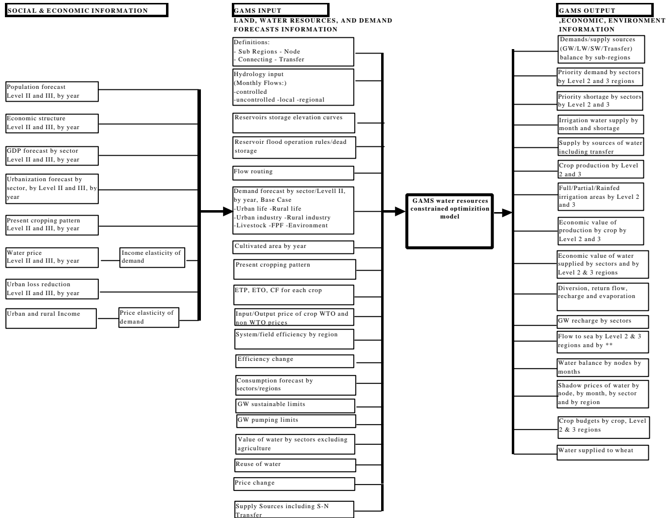
FIGURE 4.1: WATER RESOURCES CONSTRAINED OPTIMIZATION MODEL
